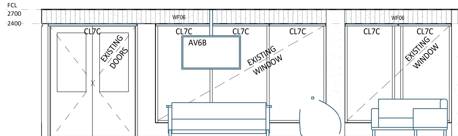
4 ELEVATION DETAIL 1 : 50
