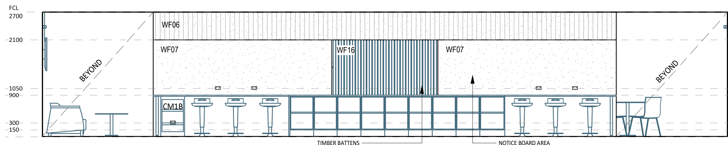
6 ELEVATION DETAIL 1 : 50
