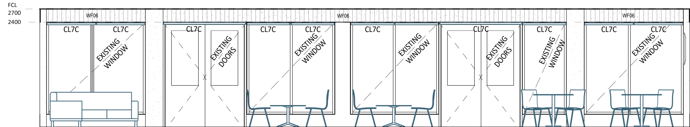
2 ELEVATION DETAIL 1 : 50
